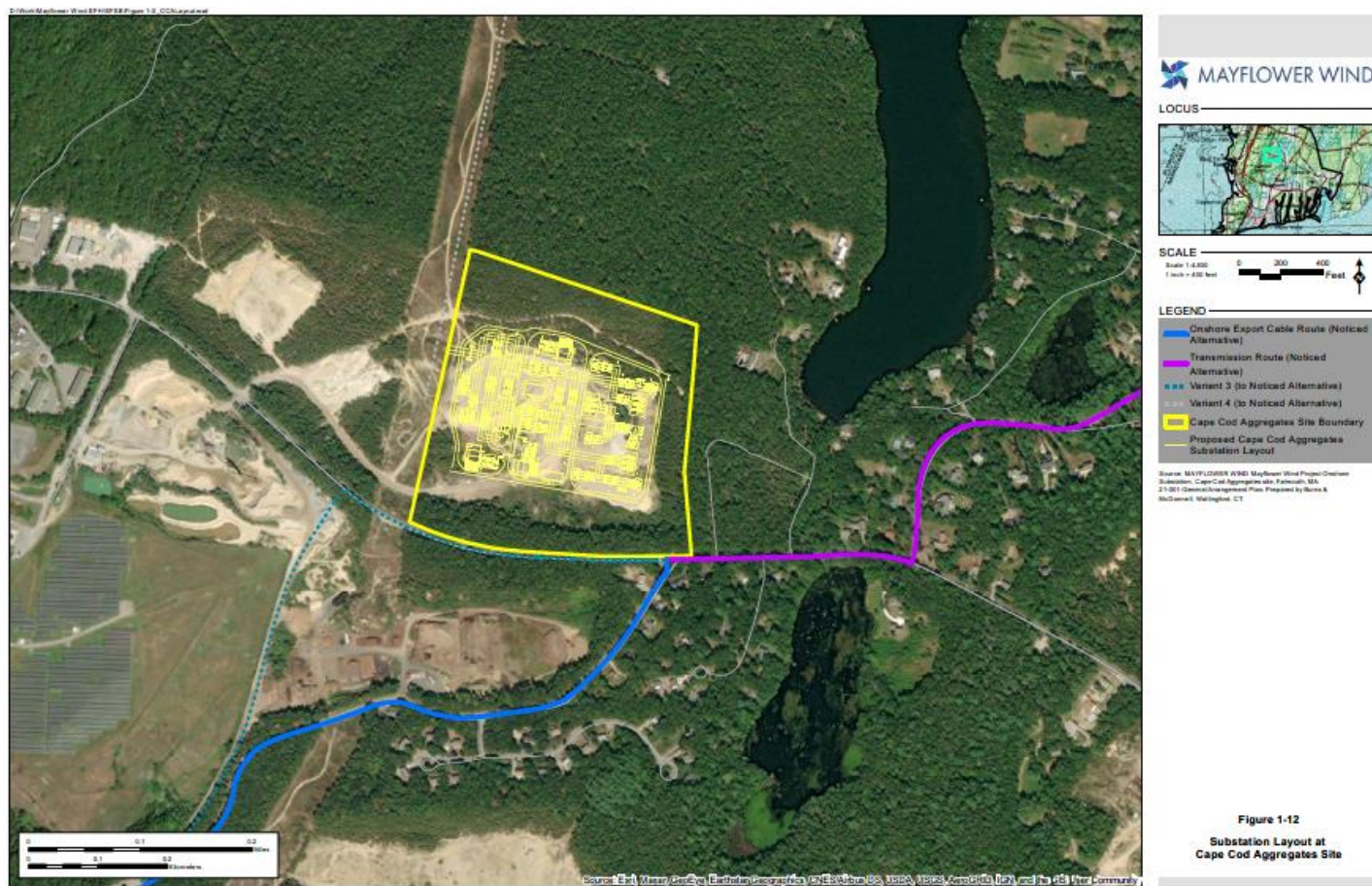
Figure 3: Mayflower Wind Project – Onshore Routes, New Onshore Substation (Noticed Alternative Route)
