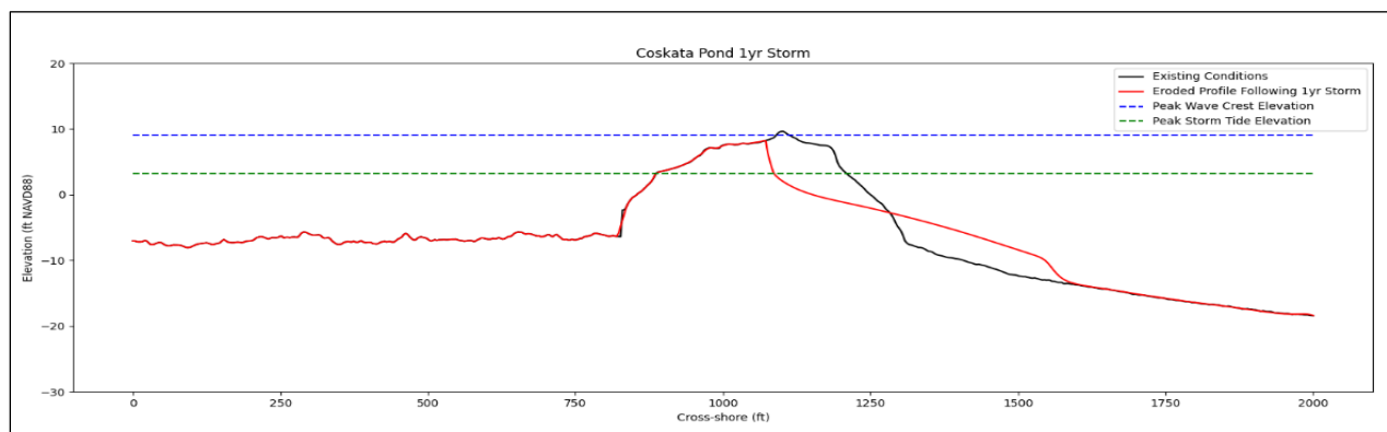
Figure 72. Caskata Pond profile after 1-year storm.
