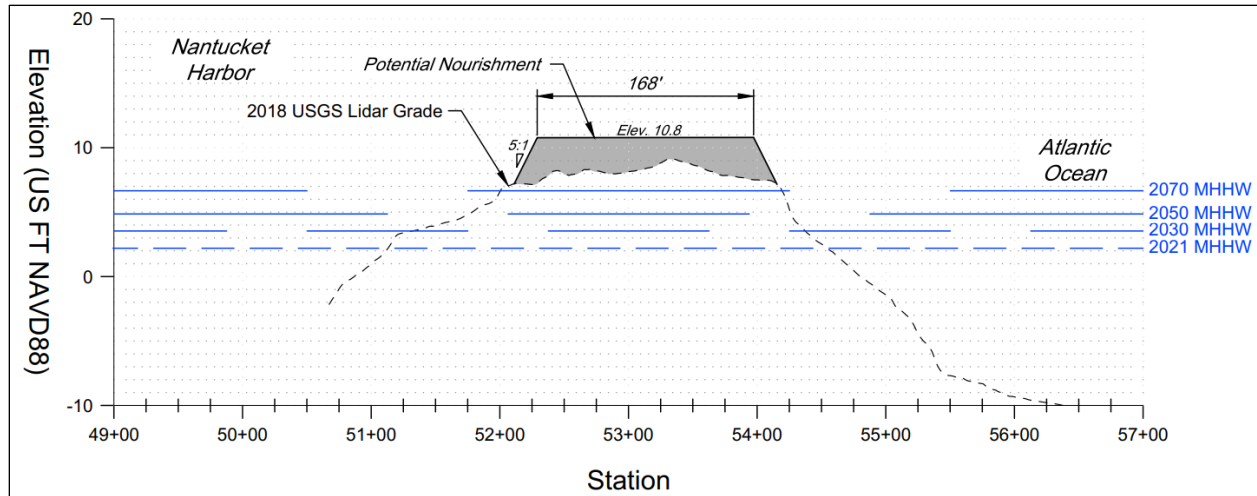
Figure 98. Conceptual dune nourishment design for Cuskata Pond.
