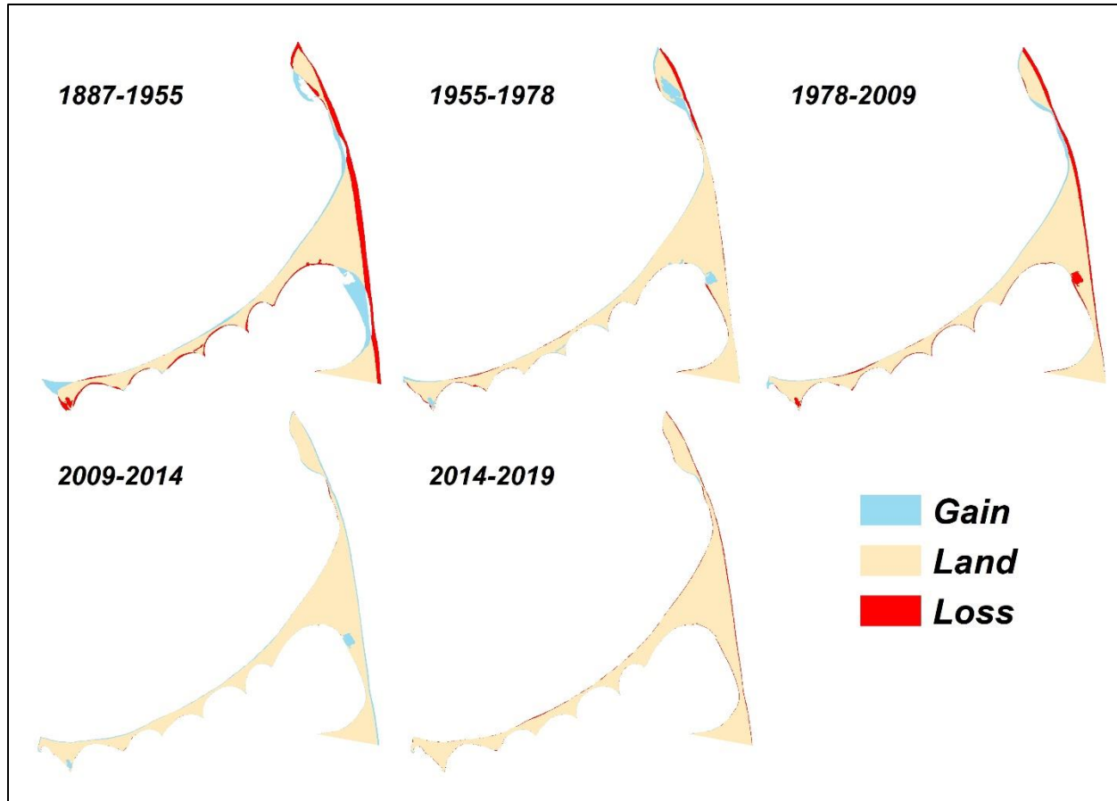
Figure 32. Incremental shoreline change for Cuskata-Coatue through time (1887-2018).
