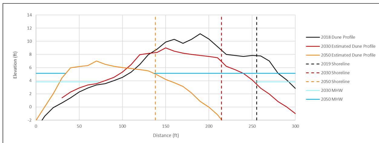
Figure 19. Recent and future dune profiles at Transect 4 east of Cuskata Pond. Shoreline positions corresponding to Figure 20 are plotted in dashed lines.
