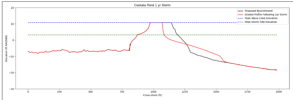
Figure 100. Conceptual nourishment and eroded profiles at Cuskata Pond during a 1-year storm.
