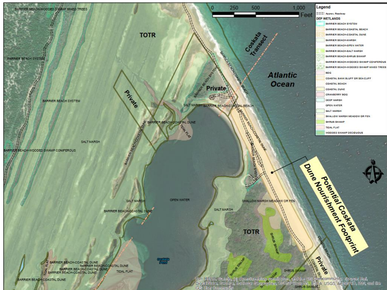
Figure 99. Potential Cuskata Pond dune nourishment footprint.
